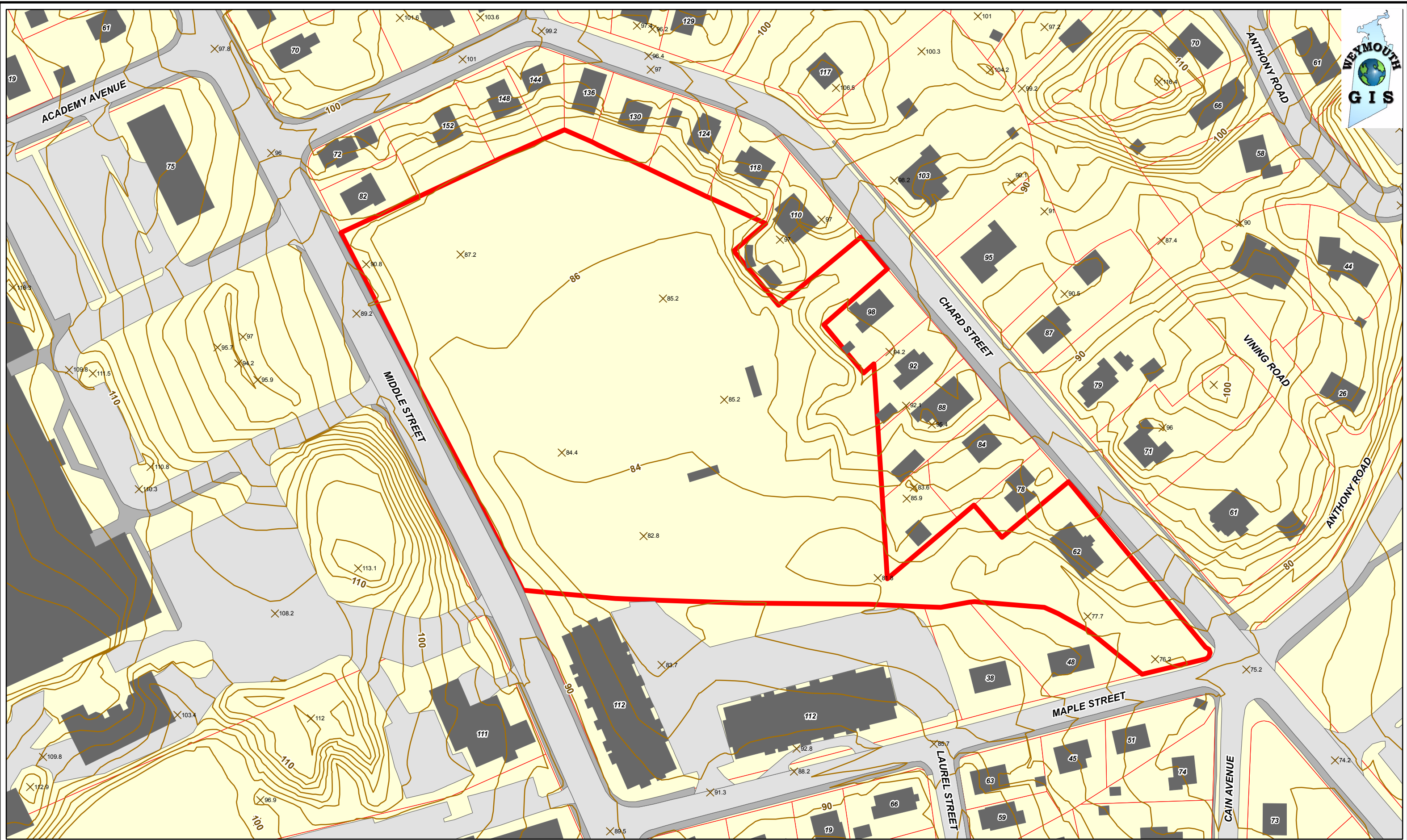
Libby Park Block 240 Lot 21 - with Topography (2 ft contours)
