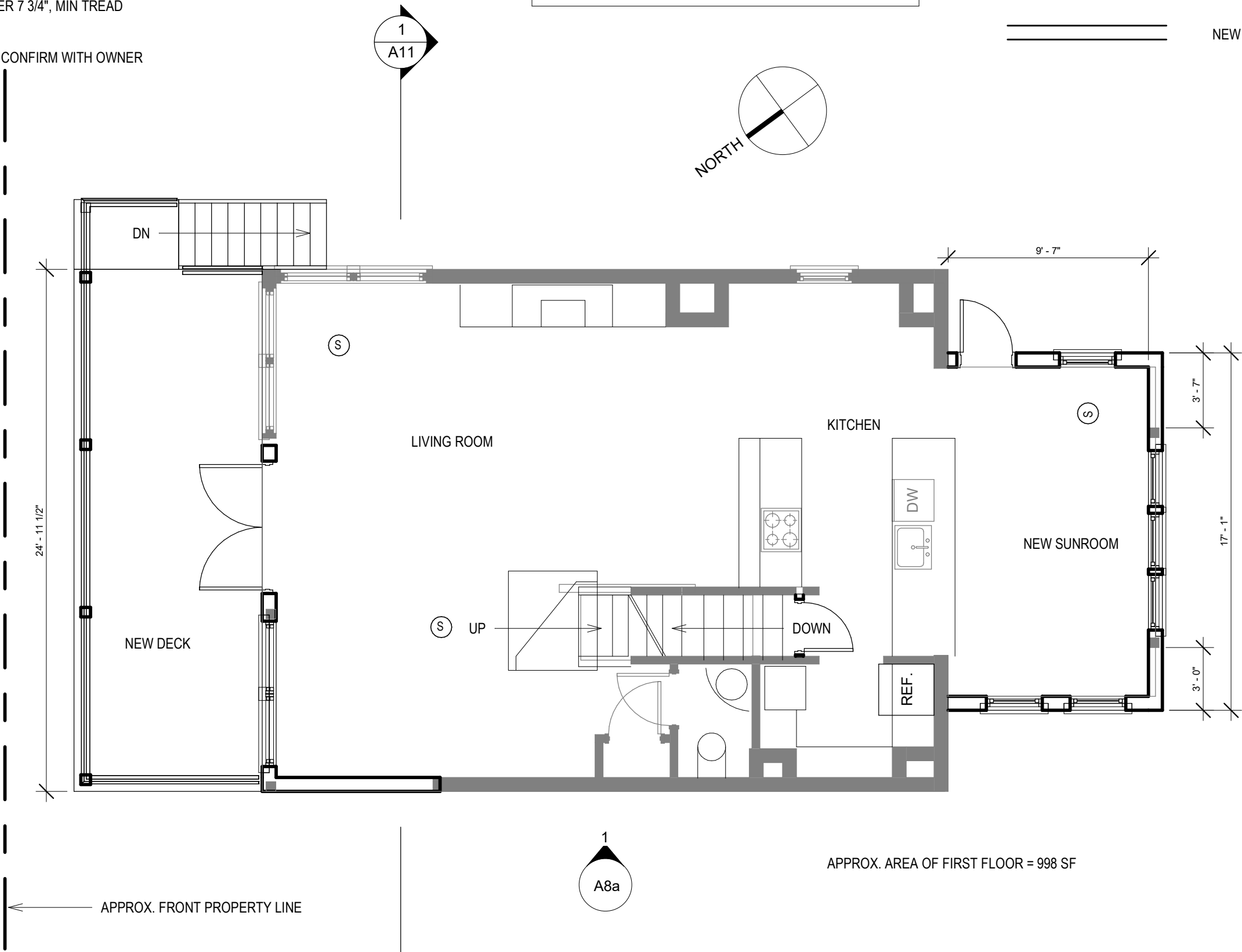
1 LEVEL 1 FLOOR PLAN NEW WORK A2 Scale: 3/16" = 1'-0" Ref: A7
