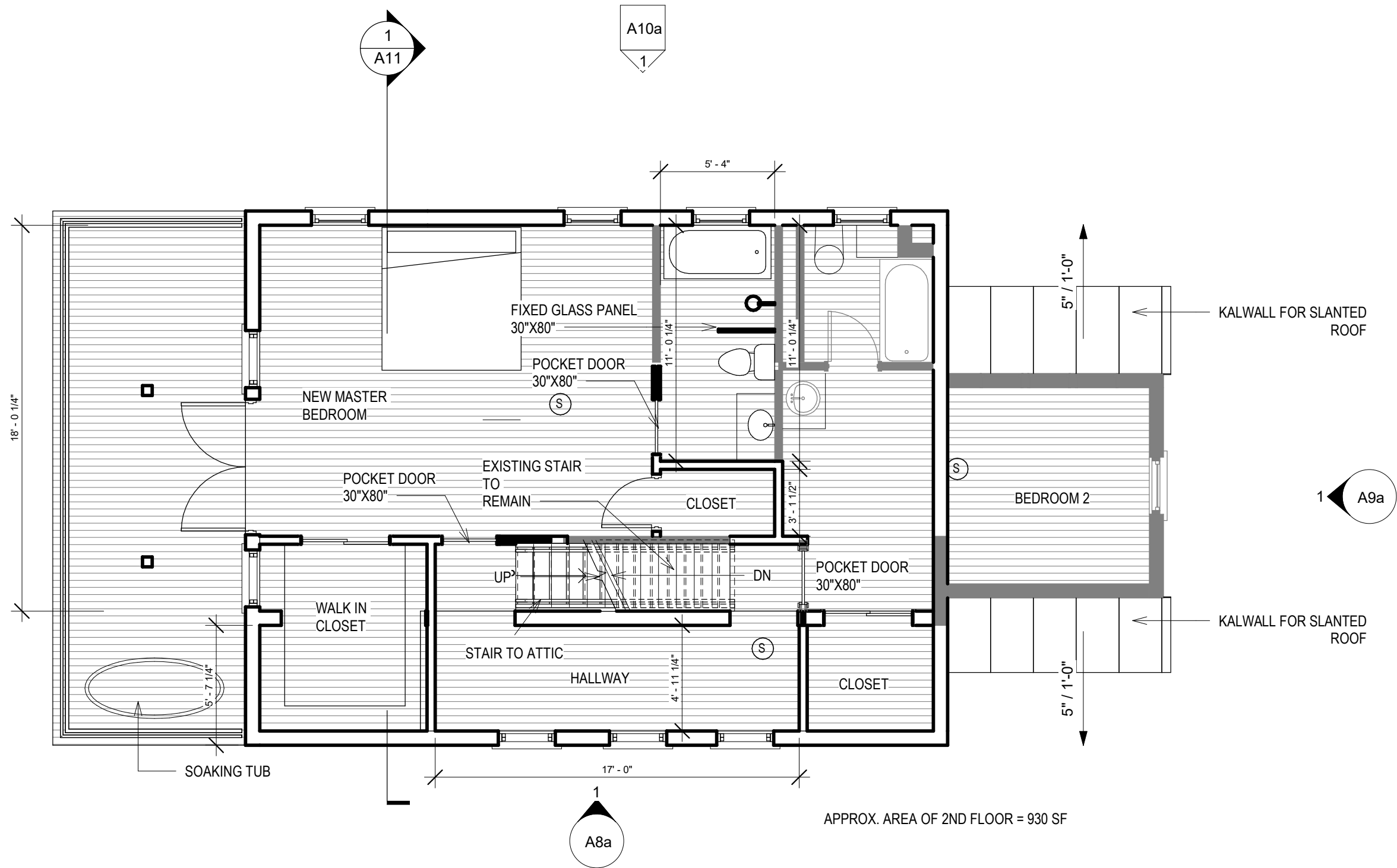
1 A3 LEVEL 2 FLOOR PLAN PROPOSED CONCEPT Scale: 3/16" = 1'-0"
