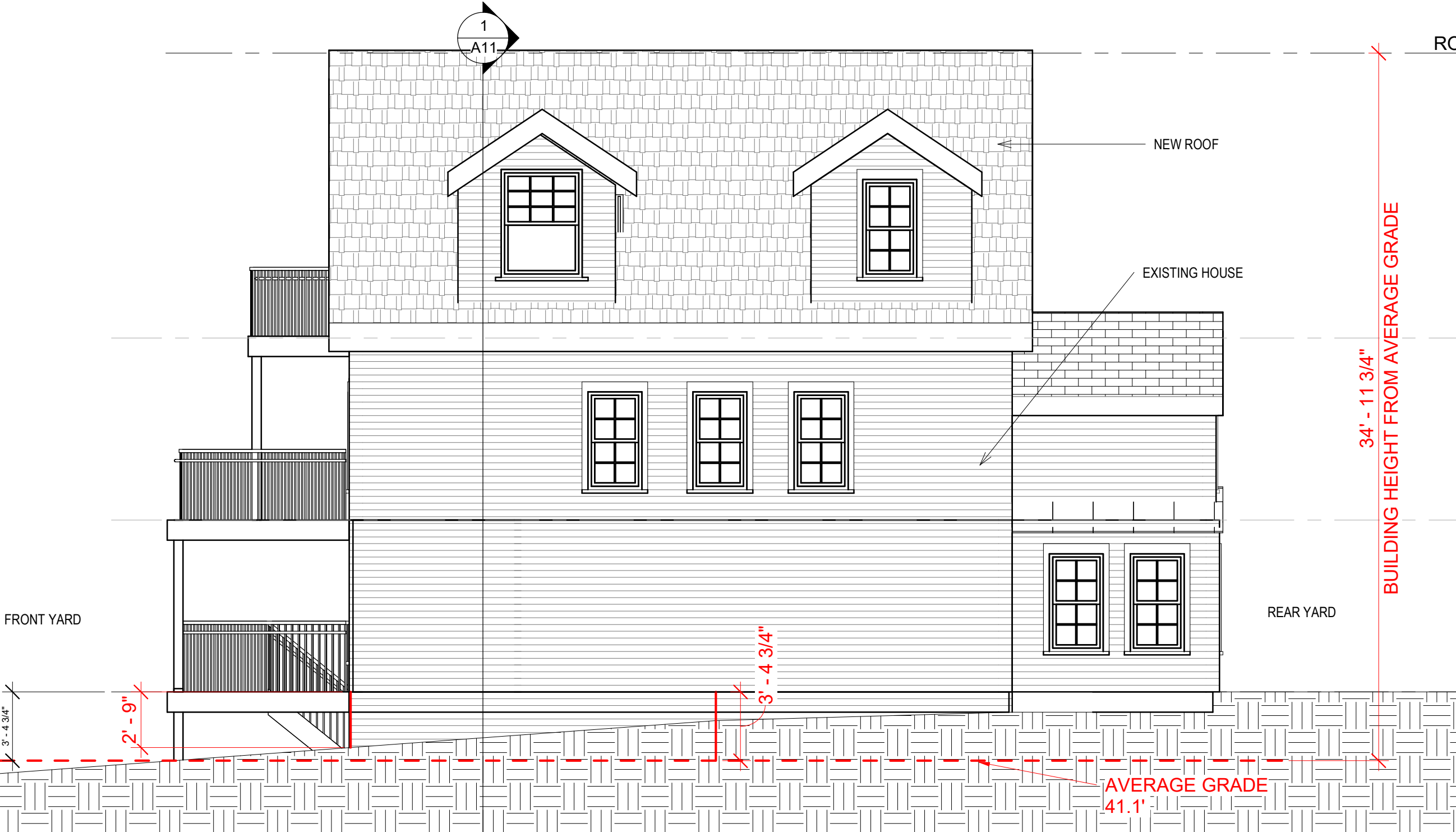
RIGHT ELEVATION - PROPOSED Scale: 3/16" = 1'-0"
